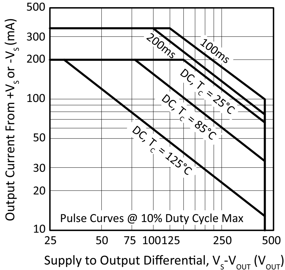
Figure 16: SOA
