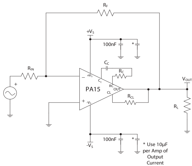
Figure 2: Typical Connection
