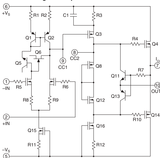
Figure 1: Equivalent Schematic
