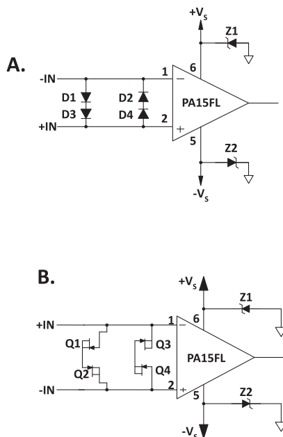
Figure 18: Overvoltage Protection
