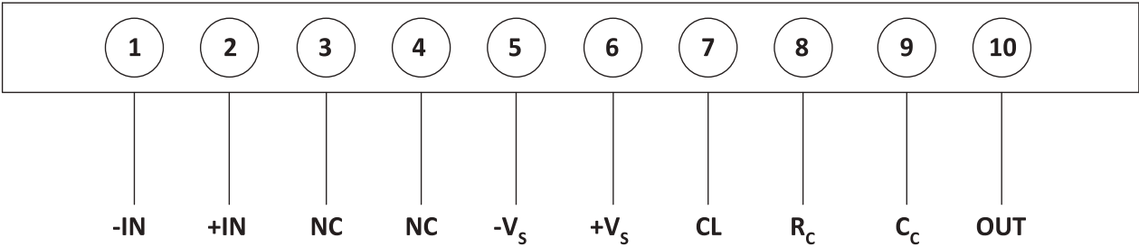
Figure 3: External Connections
