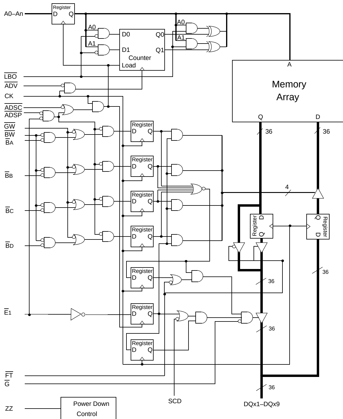
GS816218/36D Block Diagram
