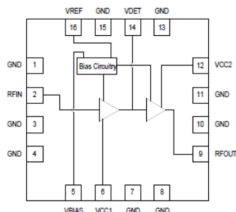
Figure 2. GSM0724 Function Block Diagram
