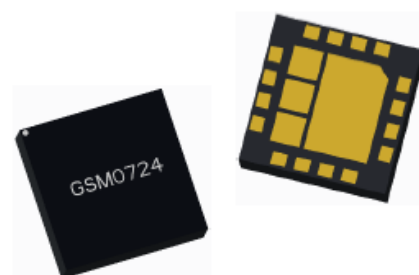
Figure 1. 16 Pad 5 x 5 mm Laminate Package
