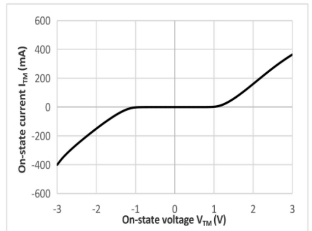
Fig.2 On-state characteristic diagram
