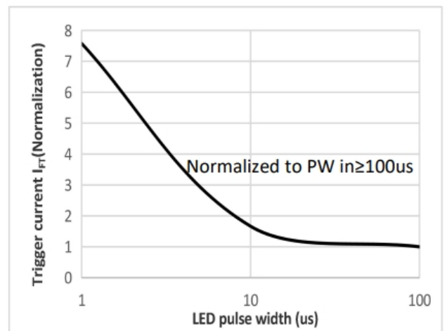
Fig.4 Trigger current vs LED pulse width
