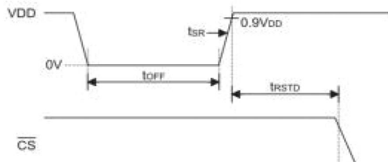
Figure 4 Power-on Reset Timing
