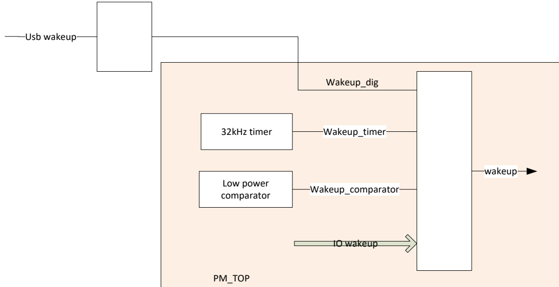
Figure 2- 6 Wakeup sources
