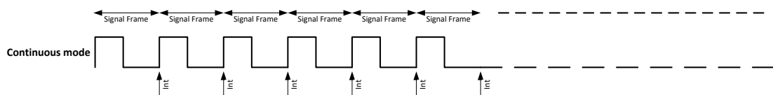
Figure 8-3 Continuous mode
