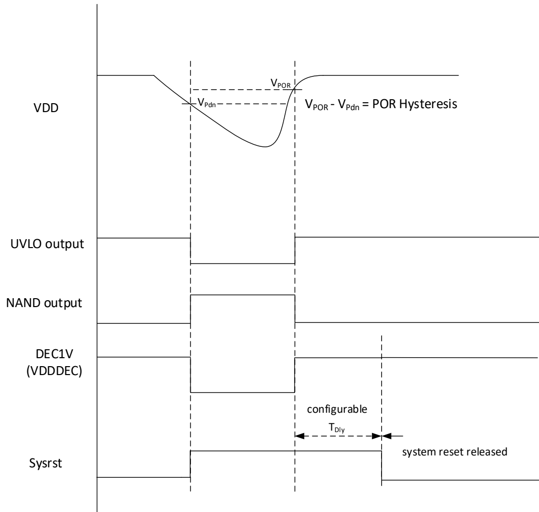
Figure 2- 5 Power-down sequence
