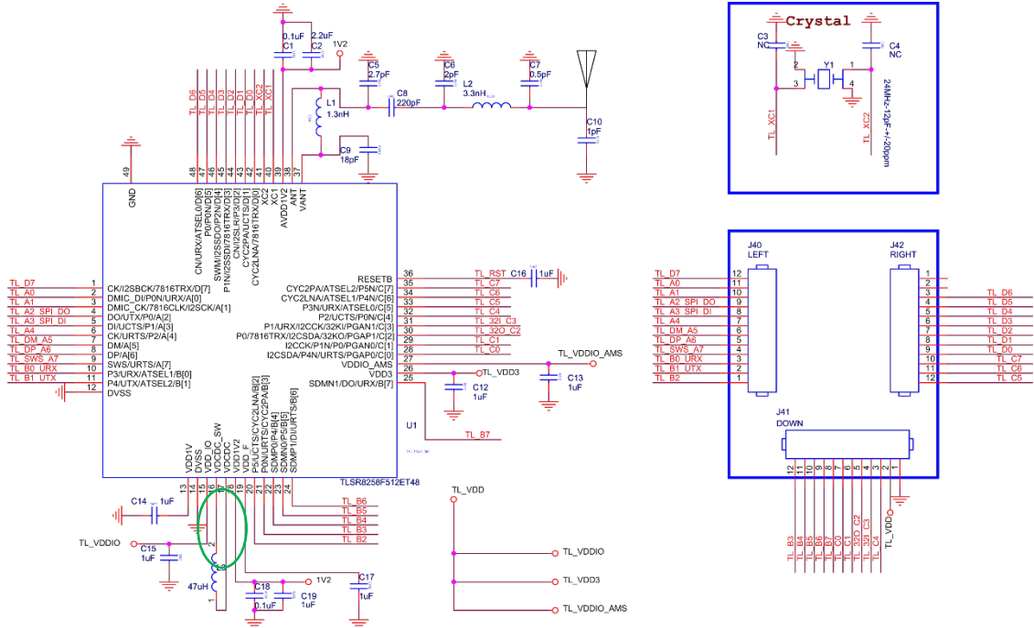
Figure 16- 1 Schematic
