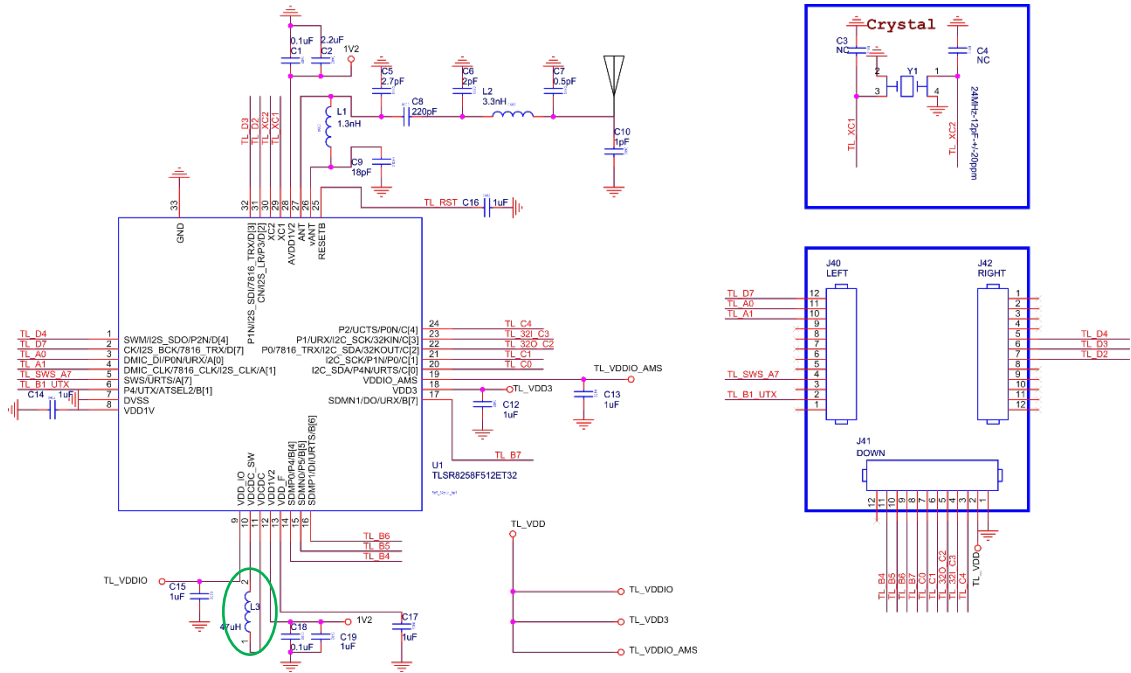
Figure 16- 2 Schematic
