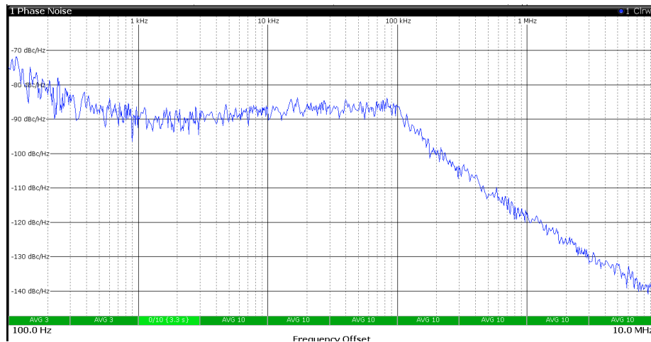
Figure 14 Phase noise plot of 3.6GHz RF PLL, I_{\text{cp}} = 400\mu\text{A} , F_{\text{Comp}} = 38.4\text{MHz} , using internal VCO, 60kHz loop bandwidth, PLL type '1100'
