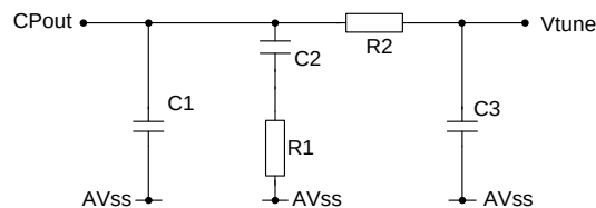
Figure 8 On-chip IF PLL Low Pass Filter Components
