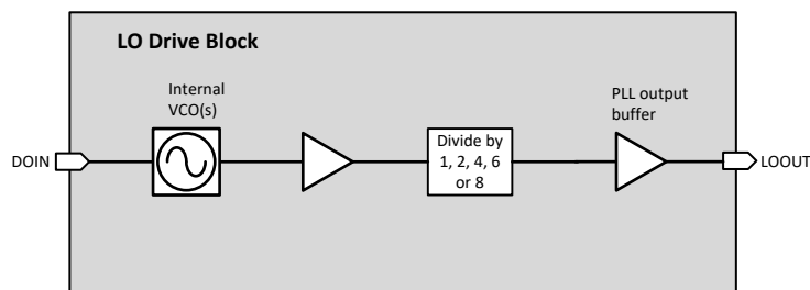
Figure 12 LO Drive Block Schematic
