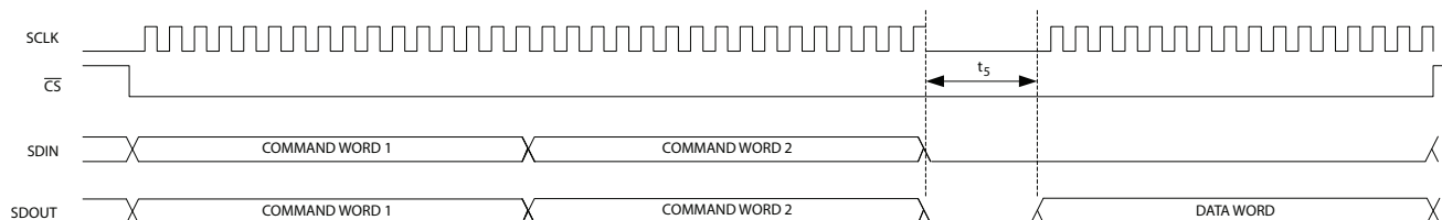
Figure 4-19: GSPI Read Timing—Single Read Access with Loop-Through Operation (default)
