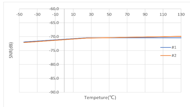
Figure 14. Signal-to-Noise Ratio vs Temperature
