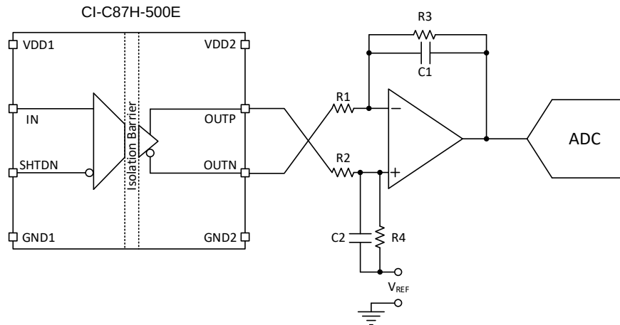
Figure 24. Connecting the CI-C87H Output to a Single-Ended Input ADC
