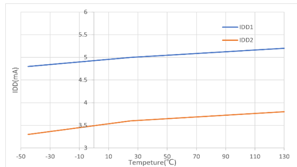
Figure 18. Supply Current vs Temperature
