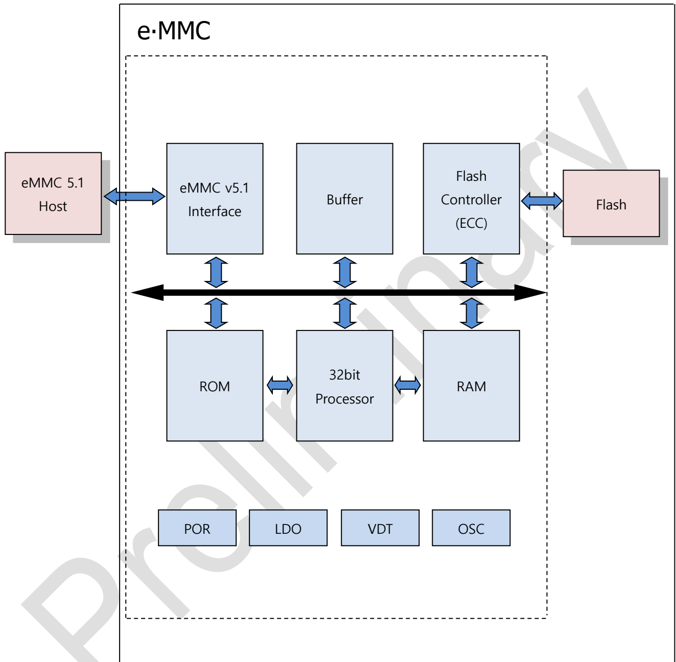
Figure 1 - e-MMC Block Diagram
