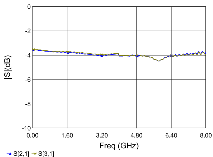
Figure 3. MPD0780W2 Insertion Loss
