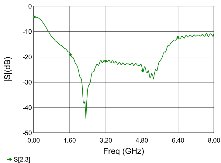
Figure 5. MPD0780W2 Isolation
