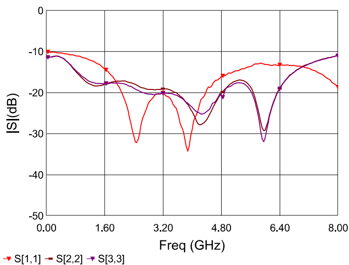
Figure 4. MPD0780W2 Return Loss
