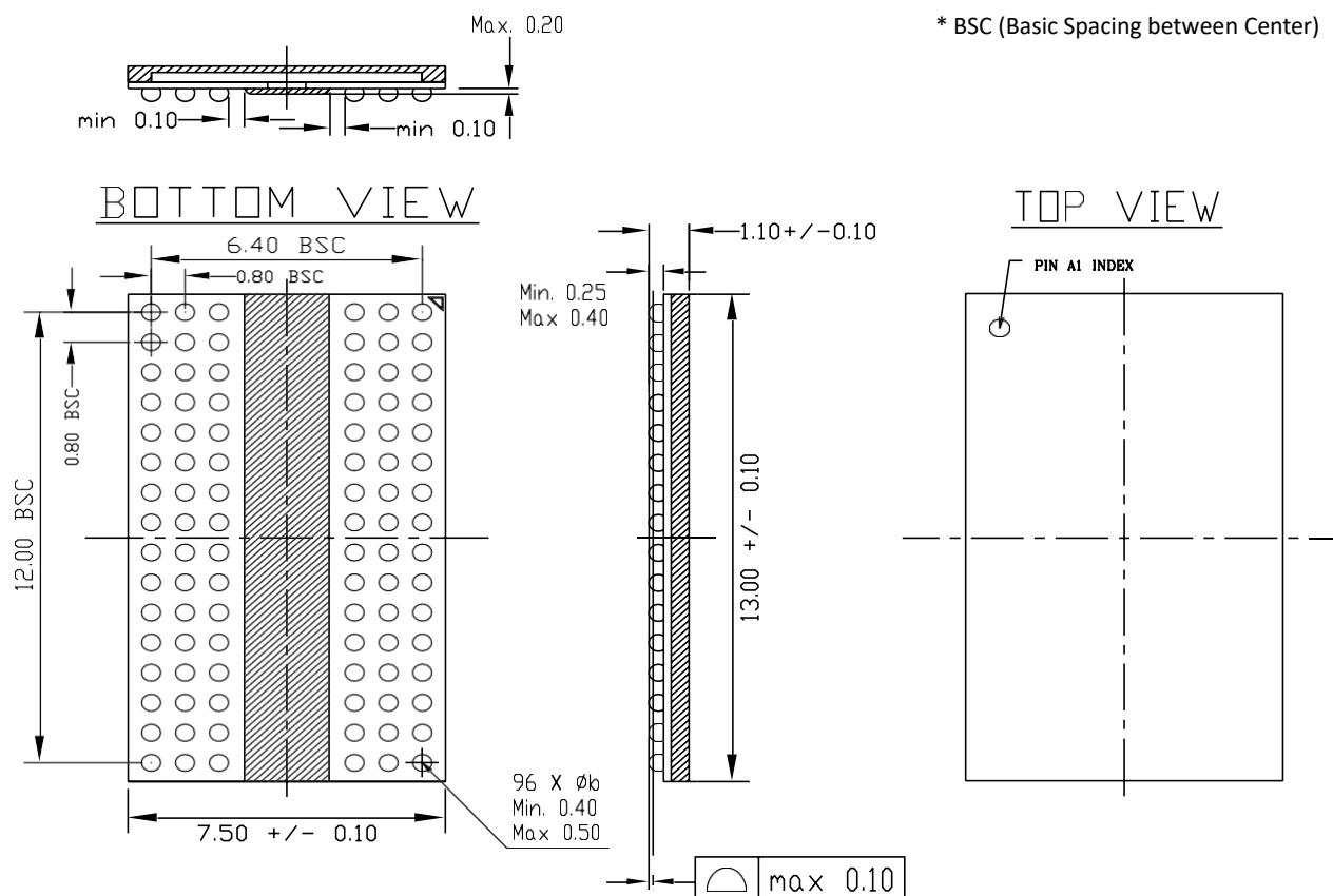
Packge Outline Drawing
