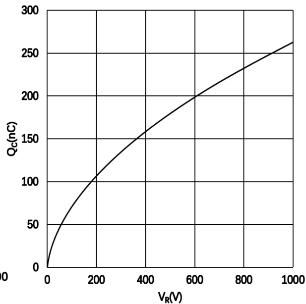
Figure 4. Recovery Charge vs. Reverse Voltage
