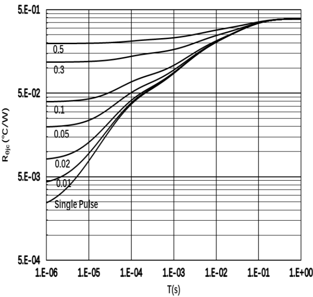
Figure 7. Transient Thermal Impedance
