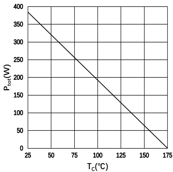
Figure 6. Power Derating
