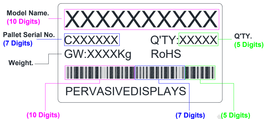
Figure 9-3 Carton Label
