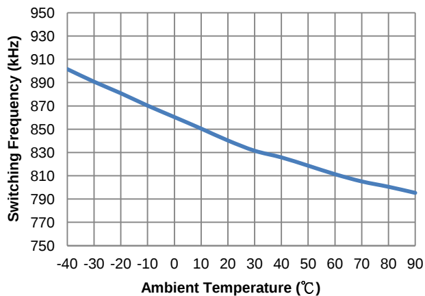
Figure 8. Switching Frequency vs. Ambient Temperature
