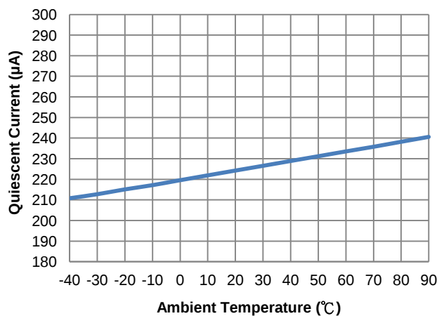
Figure 7. Quiescent Current vs. Ambient Temperature
