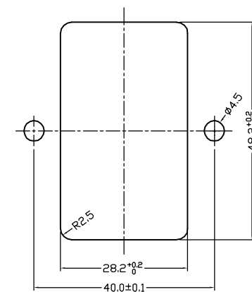
PANEL CUT-OUT
