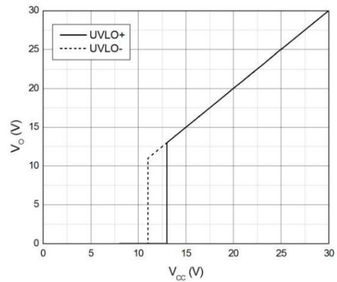
Fig.10 Output Voltage vs. Supply Voltage
