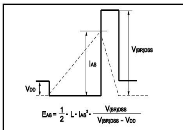
Fig.12 Avalanche Waveform
