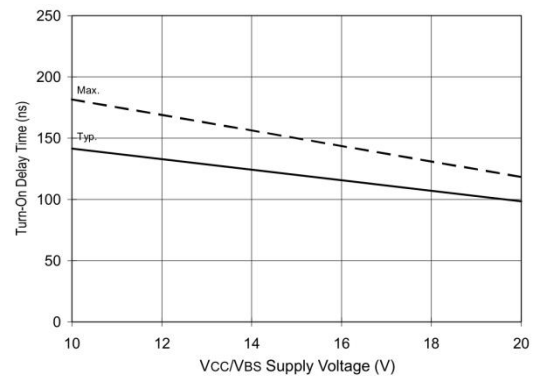
Figure 7B. Turn-On Time vs. V_{CC}/V_{BS} Supply Voltage
