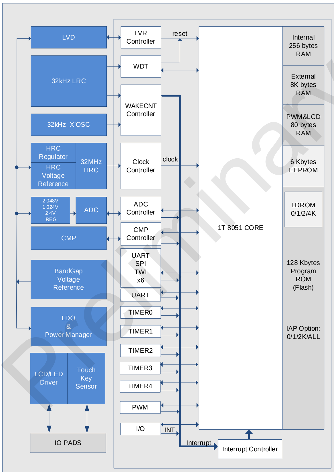
SC95F876X BLOCK DIAGRAM
