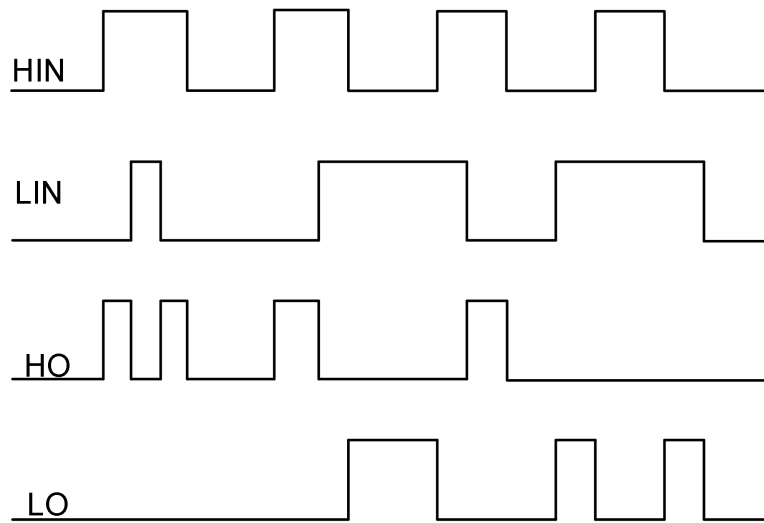
Figure 5. NSG2308 Input and output timing waveform
