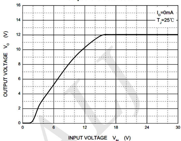
Output Characteristics
