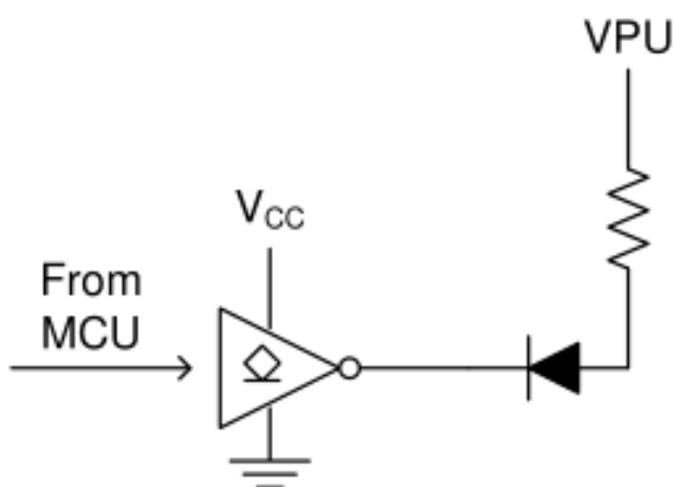
Figure 5.1: Application Schematic
