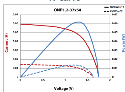
IV Curve
