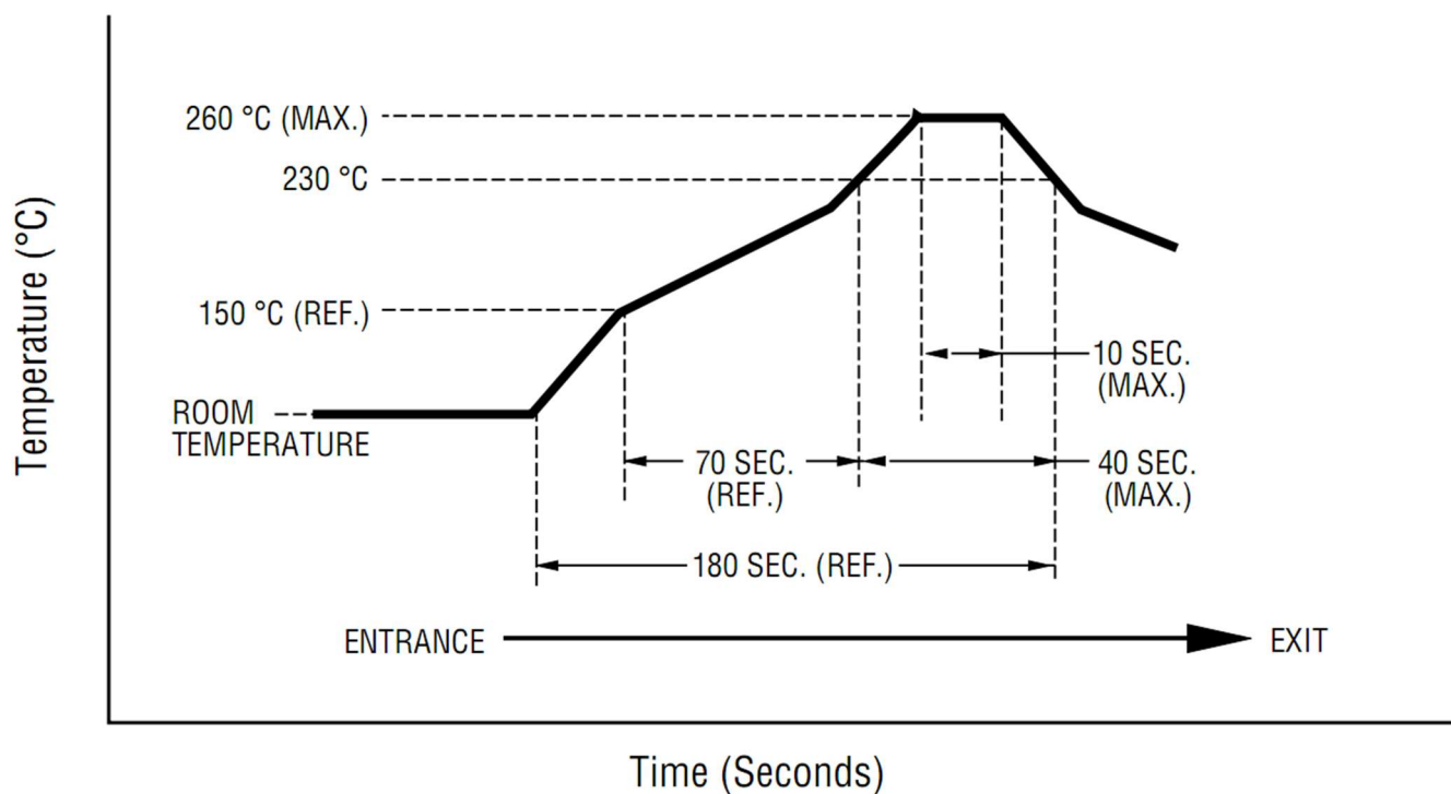
Figure 12. MHC4350L03 Thermal Reflow Profile
