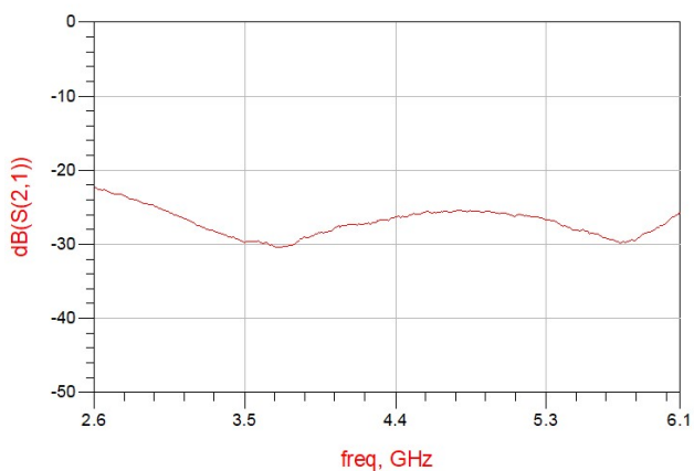
Figure 9. MHC4350L03 Isolation
