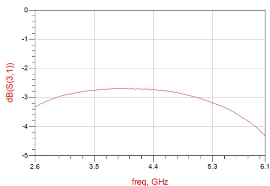
Figure 3. MHC4350L03 Coupling
