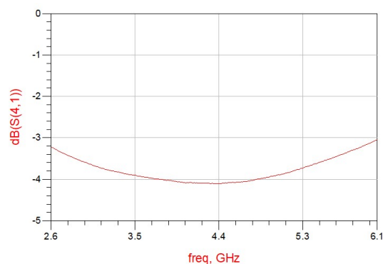
Figure 4. MHC4350L03 Transmission
