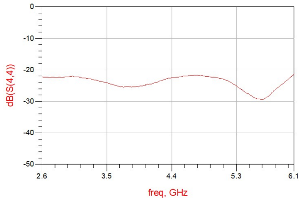
Figure 8. MHC4350L03 Return Loss (S44)
