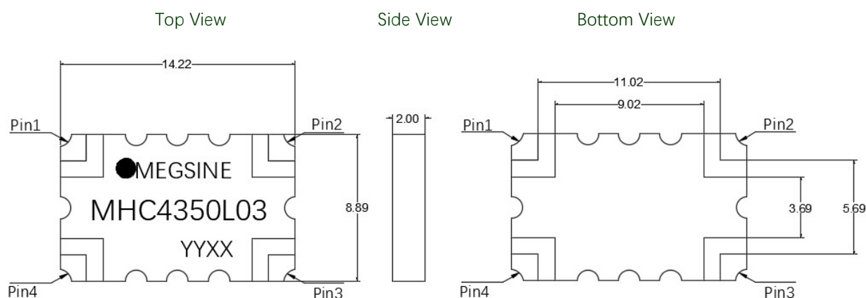
Figure 2. MHC4350L03 Outline Drawing
