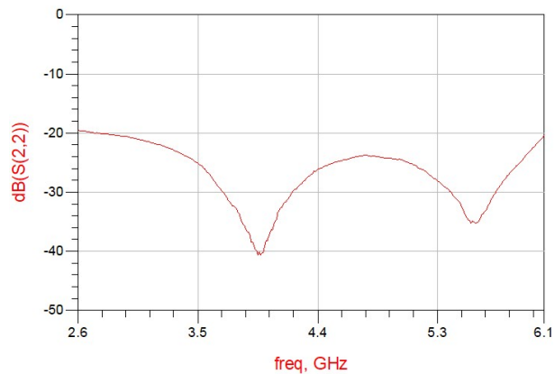
Figure 6. MHC4350L03 Return Loss (S22)
