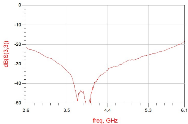
Figure 7. MHC4350L03 Return Loss (S33)
