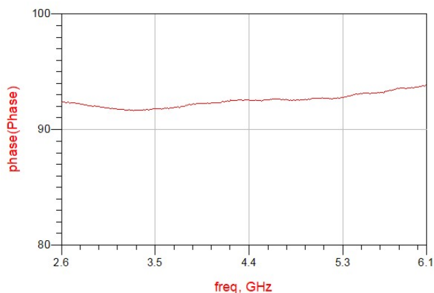
Figure 10. MHC4350L03 Phase
