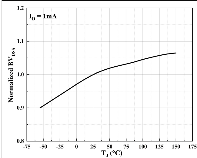
Figure 9. Normalized Breakdown Voltage vs. Junction Temperature
