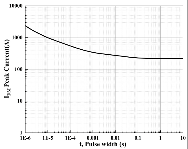
Figure 14. Peak Current Capacity
